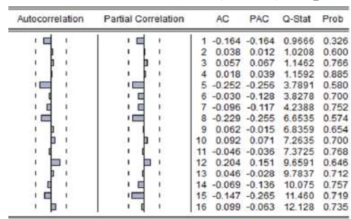
Fig. (2) : Autocorrelation function (ACF)&Partial autocorrelation function (PACF) inspection
