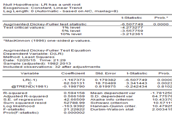
Fig. (3) : Augmented Dickey- Fuller for unit root test.
