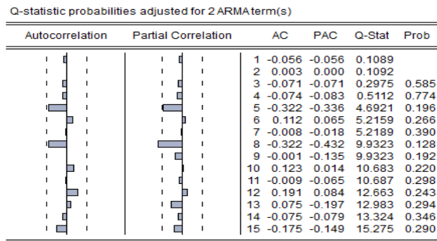
Fig. (6): Residual Autocorrelation Function Test model & Descriptive Statistics
