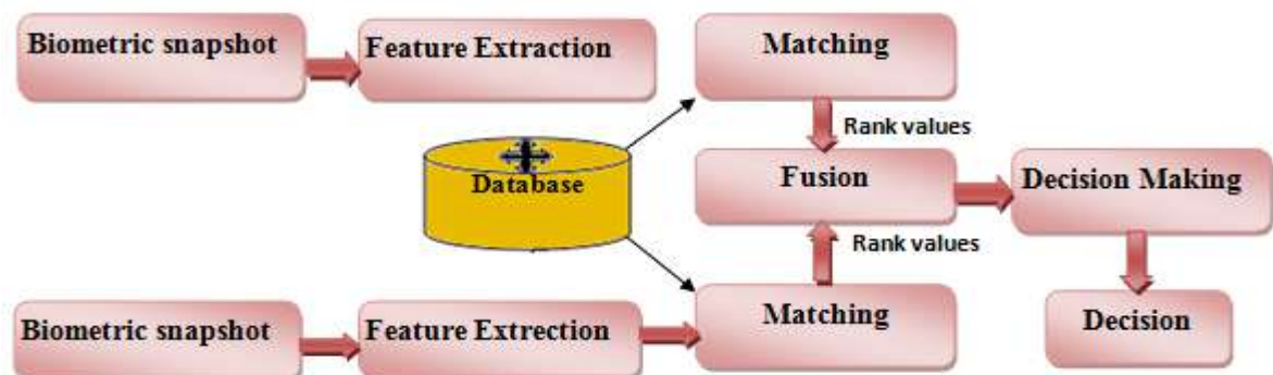
Figure I.19 Matching Score level Fusion.
