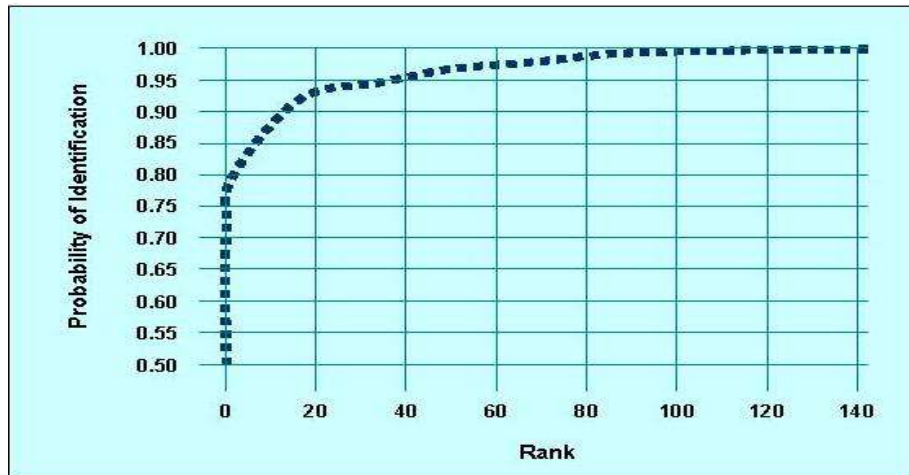
Figure I. 17 Example of CMC curve.
