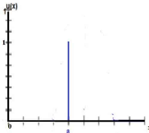
Figure II 1 singleton function.
