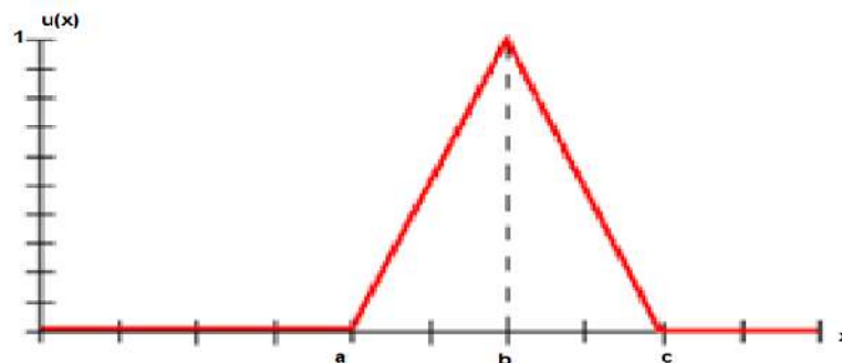
Figure II.3 Triangular function
