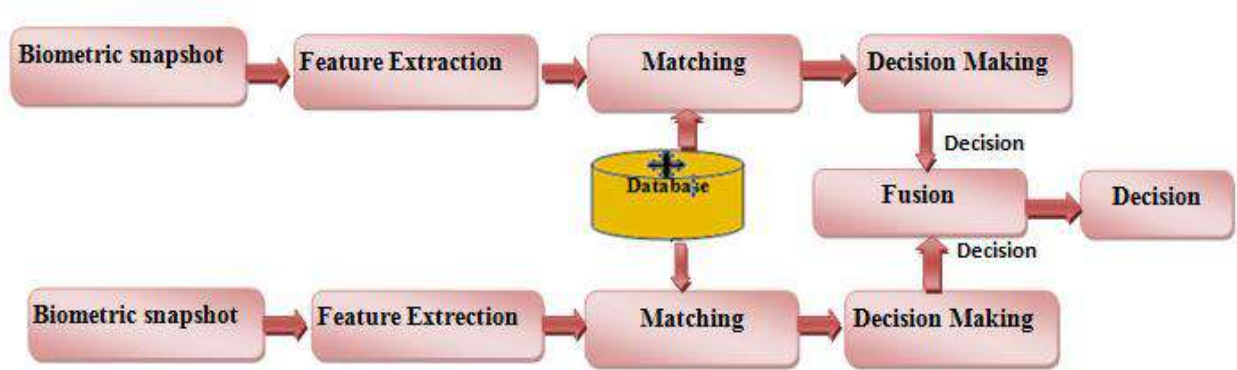
Figure I.20 decision level Fusion.
