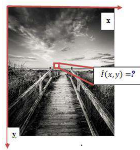
Figure II 5 Grayscale image.
