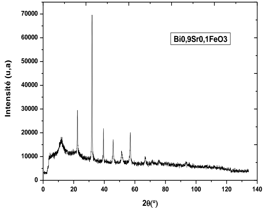
Fig. III.6: Diagramme de diffraction X de \text{Bi}_{0,9}\text{Sr}_{0,1}\text{FeO}_3
