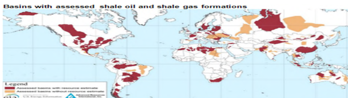
Fig 2 showing Basins with Shale oil- gas distribution including the Algerian basins (US Energy Administration source, USEIA)
