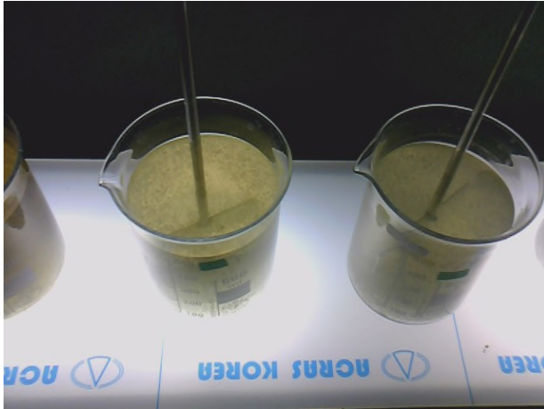
Figure 1 : jar test
