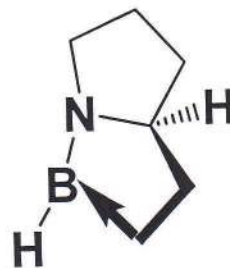
OXazaborolidines
