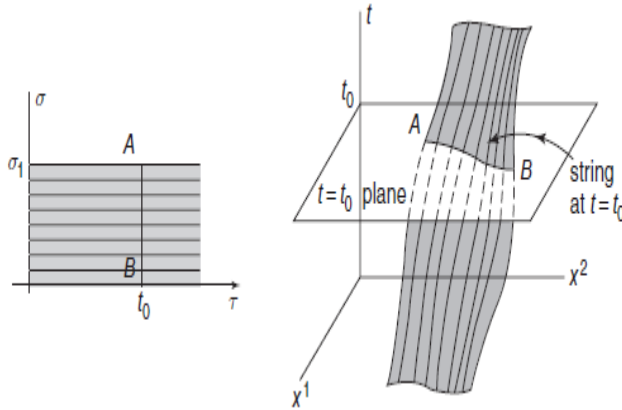
Figure 5-9. Left: the parameter space band for an open string. The vertical segment AB is the line \tau = t_0 . Right: the world map of the string open in the target space. The string at time t = t_0 is the intersection of the world leaf with the hyper plane t = t_0 . In the static gauge, the string at time t = t_0 is the image of \tau = t_0 segment AB.
