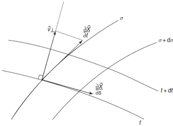
Fig5-12 a small piece of the world leaf showing the vector \frac{\partial \vec{X}}{\partial t} , the transverse velocity \vec{v}_\perp and the unit vector \frac{\partial \vec{X}}{\partial s} .
