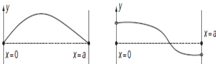
Fig. 5-8 Left: strings with boundary conditions of Dirichlet at the ends. Right: string with Neumann boundary conditions at the ends
