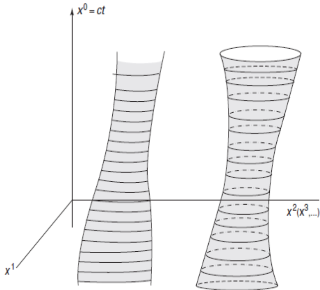
Figure- 5.1- the leaves of the world drawn by an open string (left) and a closed string (right)
