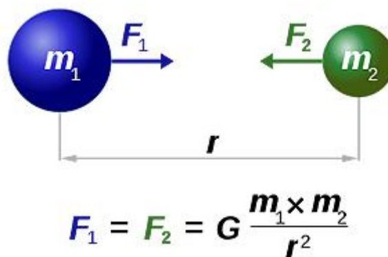
figure 2.1 : The gravitational interaction of two spherical bodies according to Newton[13]
