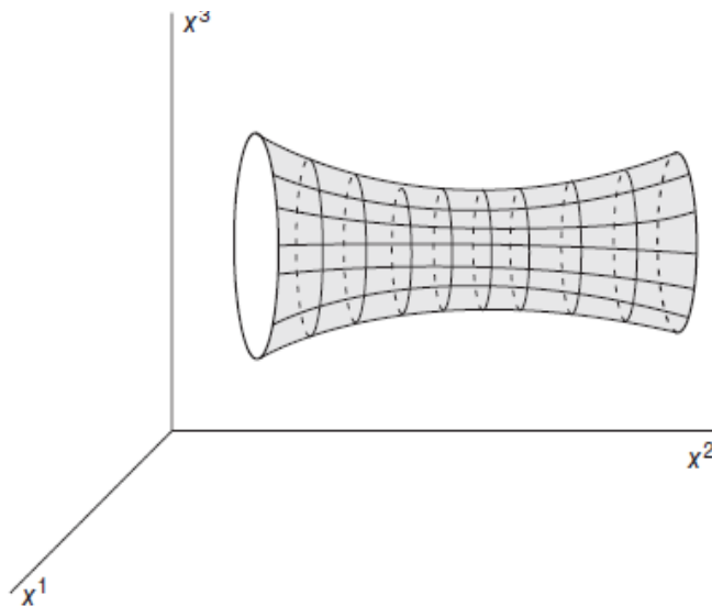
Figure- 5.2 - Area a space stretch between two rings. If the surface exists in its entirety at any time of the deadline.
