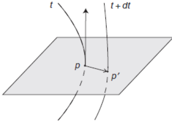
Figure 5-11 A string at time t and the point orthogonal to the string at p . At the instant +dt , the string cuts the plane in p' . To define the transverse velocity, we assume that p has passed to p' .
