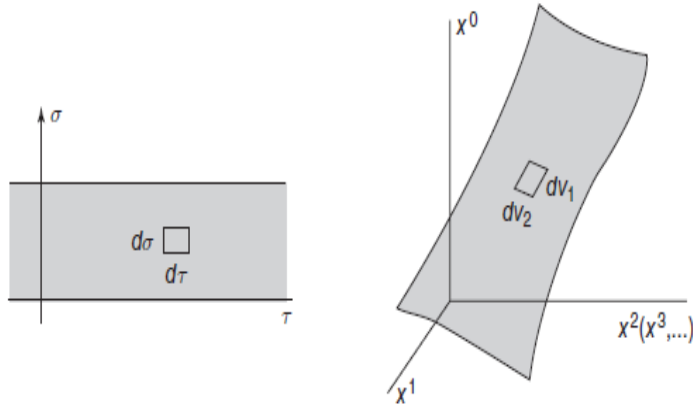
Figure 5.4 Left: the parameter space ( \tau , \sigma ), with a small square selected. On the right: the surface in the target space-time with the image of the small square, a parallelogram whose sides are the vectors dV_1^\mu and dV_2^\mu
