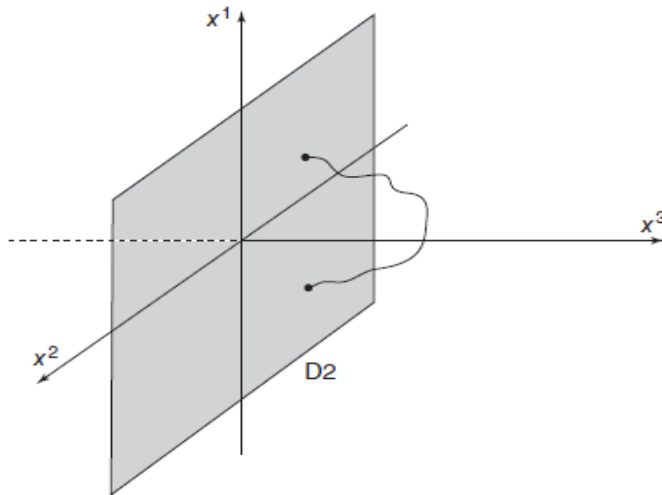
Fig5-7 A brane D2- stretched on the plane (X^1, X^2) . The end of the open string can move freely on the plane but must remain attached to it. The x^3 coordinate of the ends must disappear at any time. This is a boundary condition of Dirichlet for the string coordinate x^3 .
