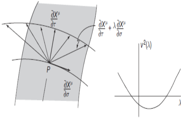
Figure 5.6: On the left: a set of tangent vectors v(\lambda) at a point P on the world map. On the right: a graph of v^2(\lambda) as a function of \lambda . The vector v(\lambda) can be of spatial or timelike type depending on the value of \lambda .
