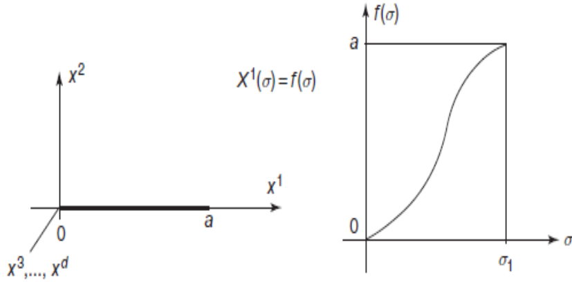
Fig.5-10. A string of length stretched along the axis X^1 . The string is parametrized as X^1(t, \sigma) = f(\sigma) .
