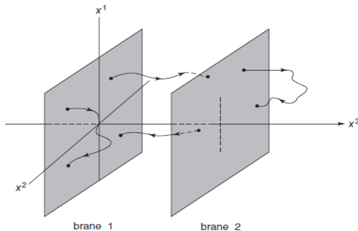
Fig-6.1. Two D2- parallel branes. Here x^1 and x^2 are longitudinal coordinates, and x^3 is a normal coordinate. The positions of brane 1 and brane 2 are specified by the coordinates \bar{x}_1^3 and \bar{x}_2^3 , respectively. We show the four types of strings that this configuration supports.
