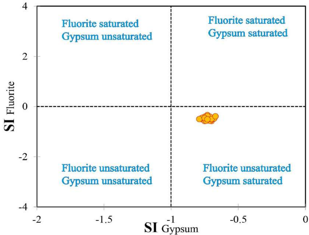
Figure 88: Diagrammes de fluorite (SI)vs gypse (SI).
