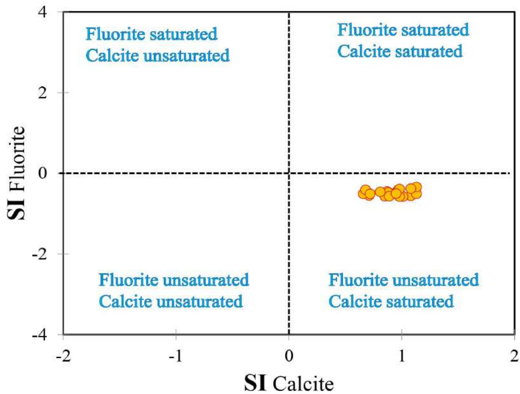
Figure 86: Diagrammes de fluorite (SI)vs calcite
