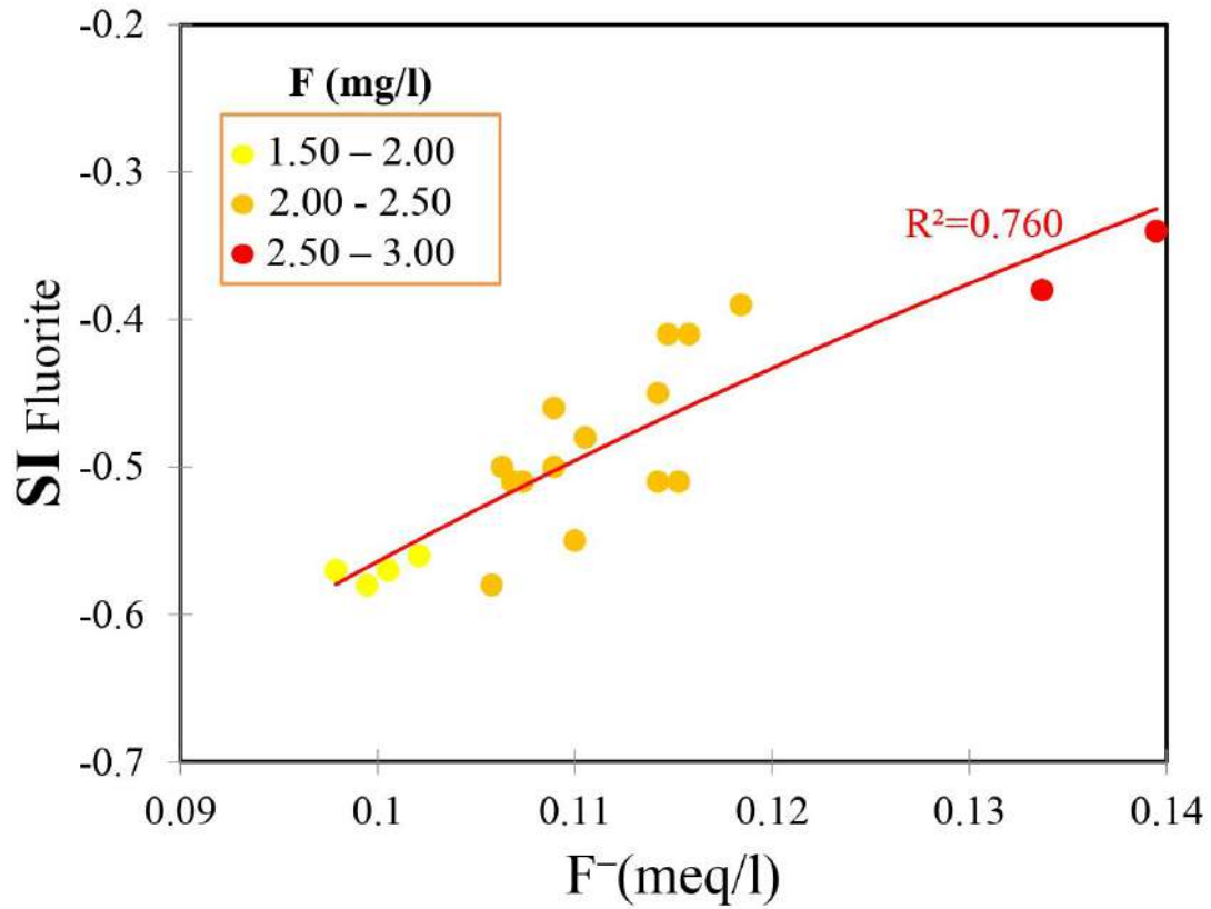
Figure 85: Diagrammes de fluorite (SI) vs F-
