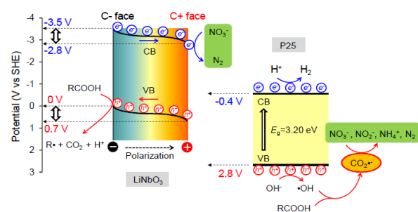
Figure.I.15: A scheme showing the method of removing nitrates from water using a photocatalyst \text{LiNbO}_3 [123].
