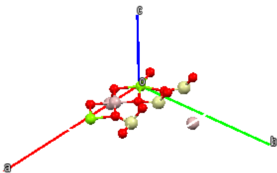
Figure.VII.11: asymetric unit
