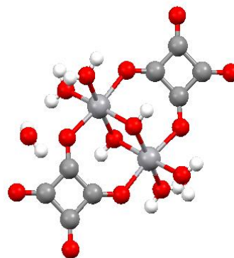
Figure.V.6: molecular unit
