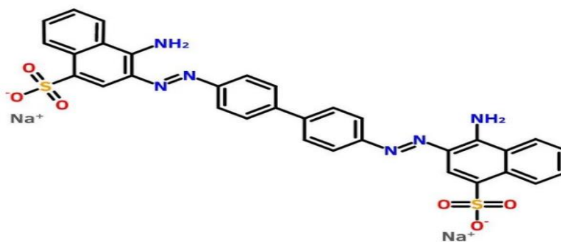
Figure I-1: Congo red structure.
