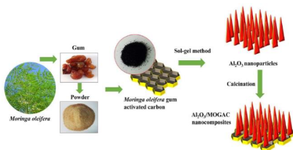
Figure.I.16: synthesis stages of aluminum oxide nanoparticles ( \text{Al}_2\text{O}_3\text{NPs} )/Moringaoleifera gum activated carbon (MOGAC)-based nanocomposites
