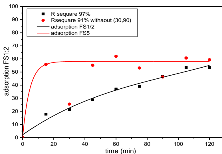
Figure.V.11: Comparaison of the two catalysts FS5 and FS12.
