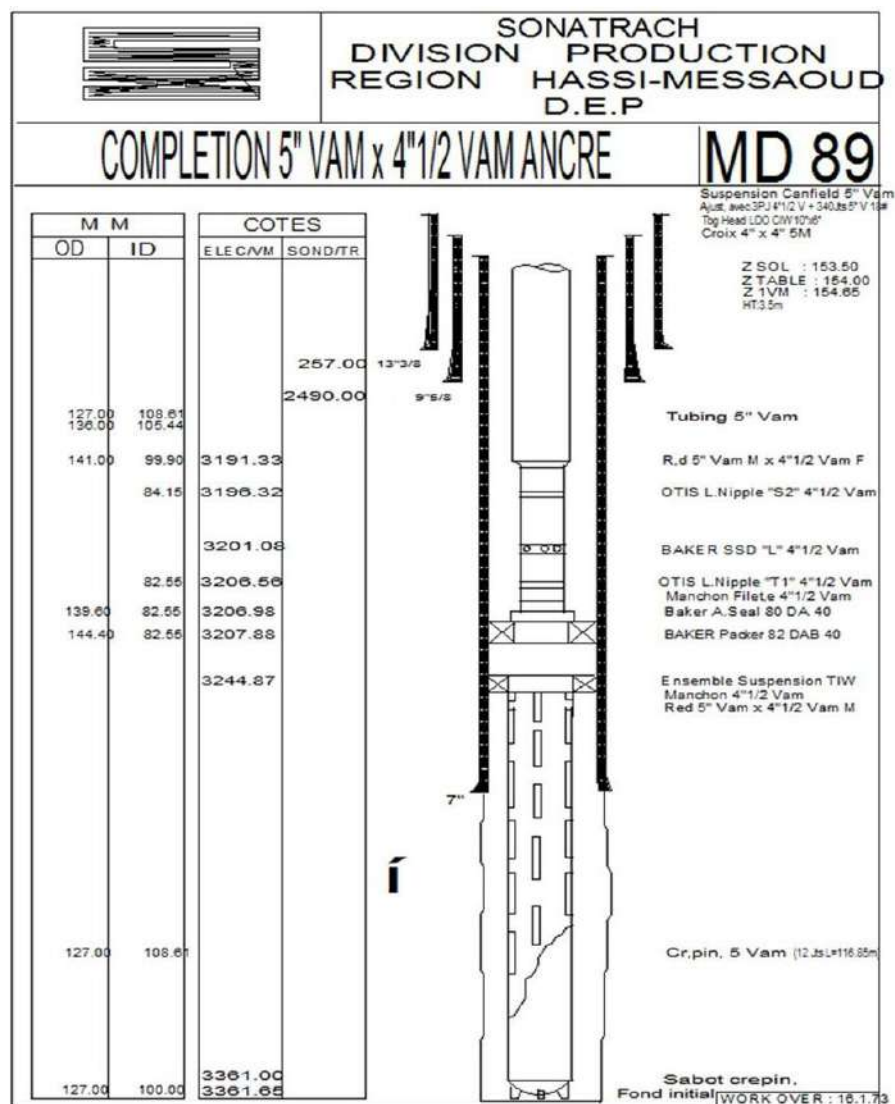
Figure III.4: Well Schematic
