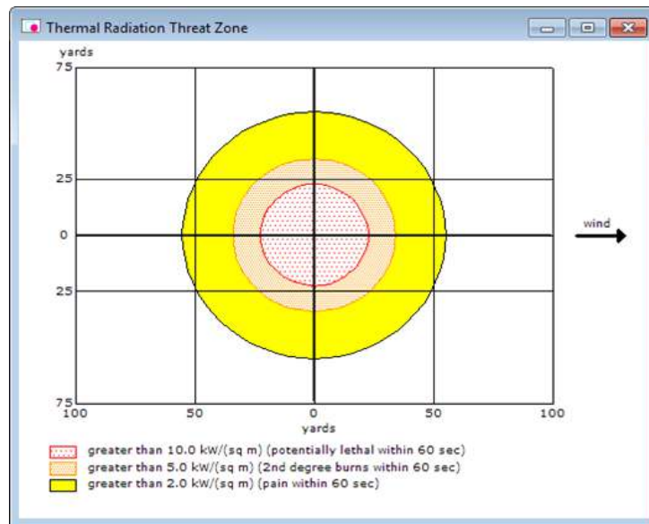
Figure II.3: Thermal Radiation LOCs
