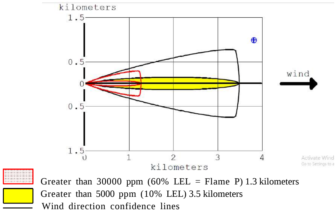
Figure III.5 Flammable LOC
