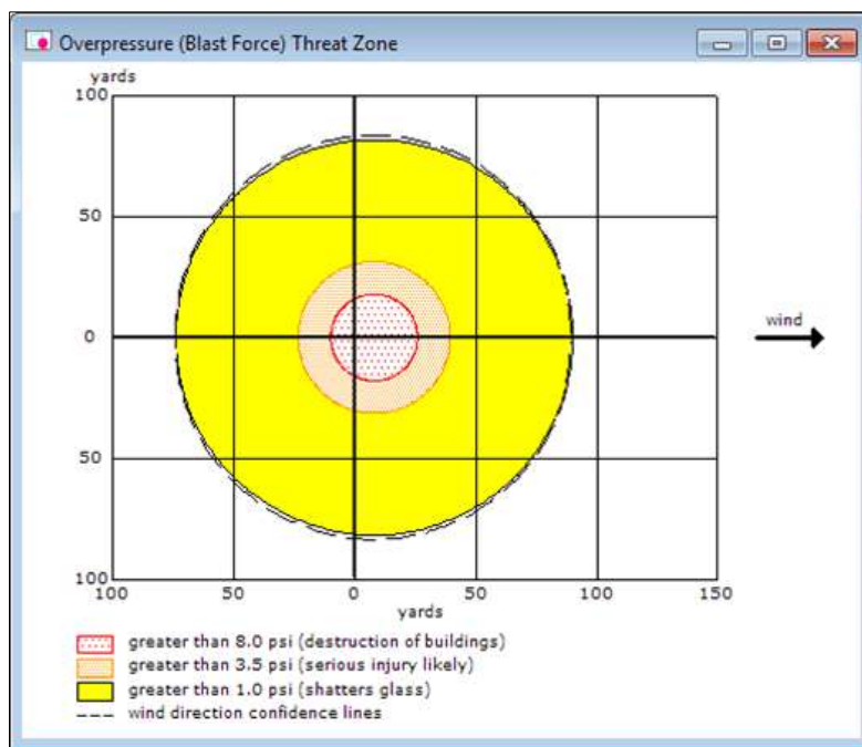
Figure II.2: Overpressure LOCs
