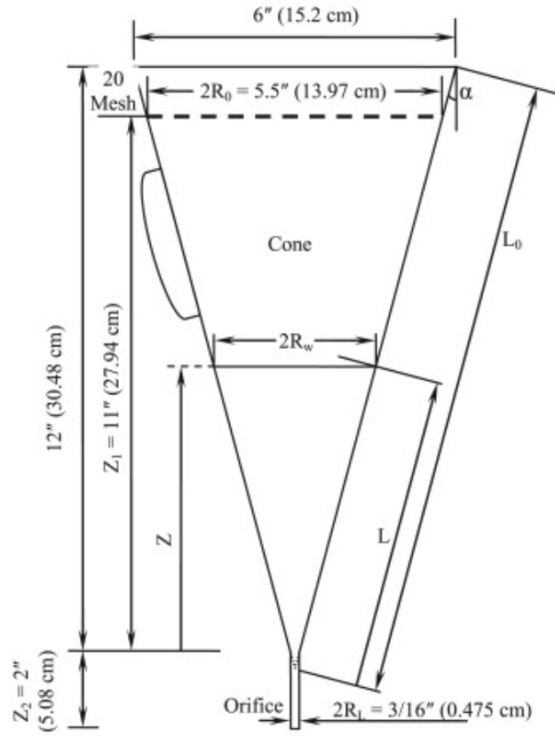
Figure 1-2 : Schematic representation of standard Marsh Funnel ( Guria, 2013 ).
