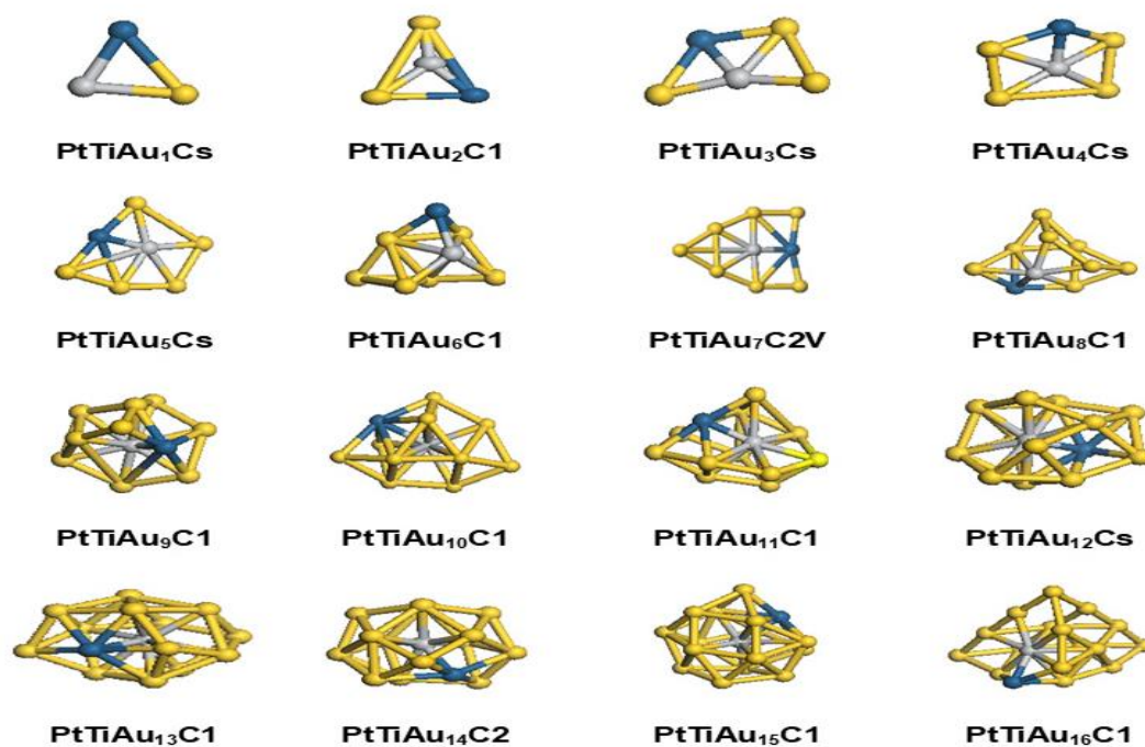
Figure 7. The most stable structures of PtTiAu_n ( n = 1-16 ) clusters.
