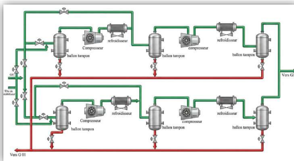
Figure II.2 : Unité boosting G05.
